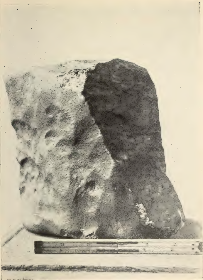
STRATHMORE METEORITE, ESSENDY FRAGMENT Photograph taken December 3, 1917, by H. Coates
